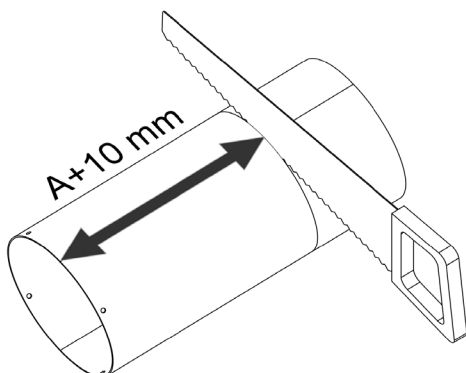
Figure 8 - Shortening of the Ø250 mm tube
